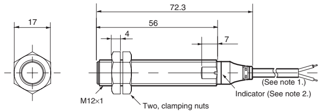
E2A-M12LS04-WP-□□
