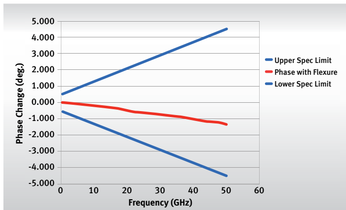
FIGURE 2: TYPICAL PHASE STABILITY WITH FLEXURE 1
