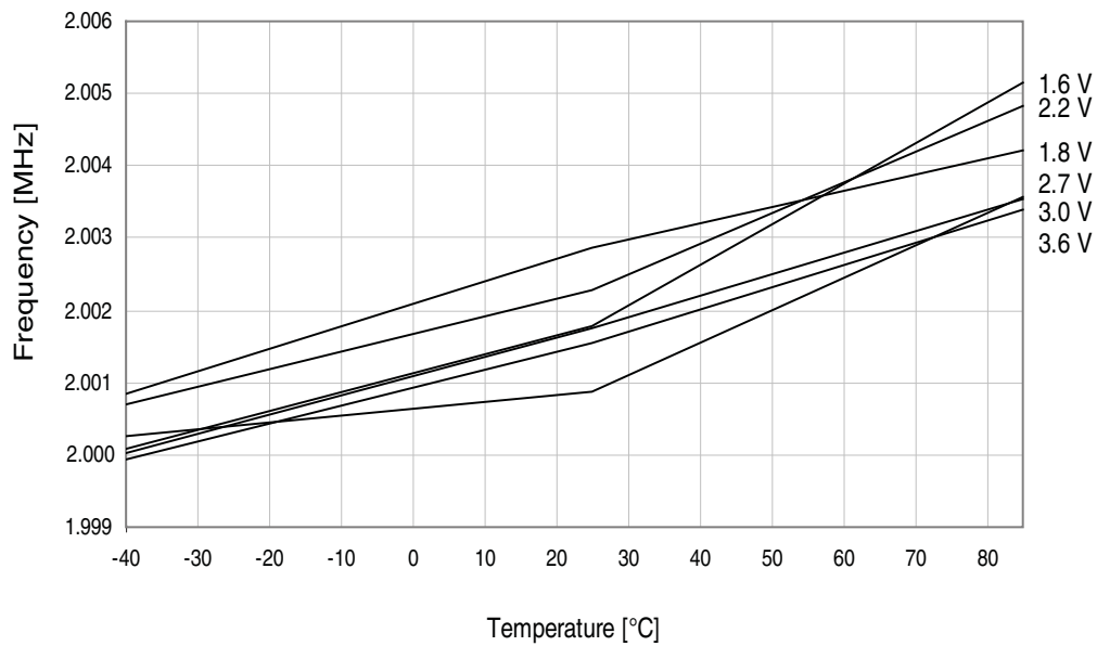
Figure 37-62. 2MHz internal oscillator frequency vs. temperature. DFLL enabled.
