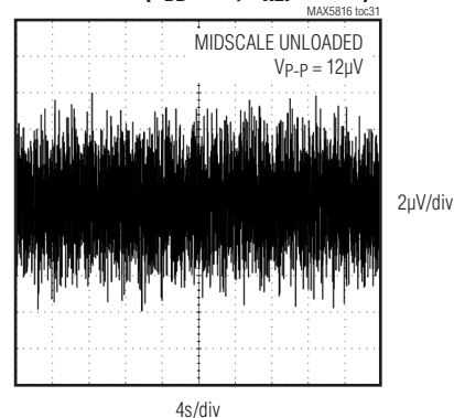
0.1Hz to 10Hz OUTPUT NOISE, EXTERNAL REFERENCE (V DD = 5V, V REF = 4.5V)
