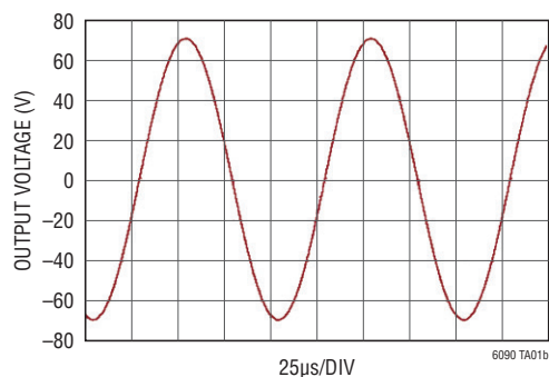
140V p-p Sine Wave Output
