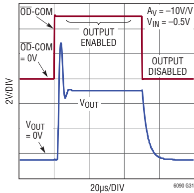
Output Disable ( \overline{\text{OD}} ) Response Time
