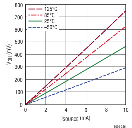
Output Voltage Swing High ( V_{\text{OH}} ) vs Load Current and Temperature
