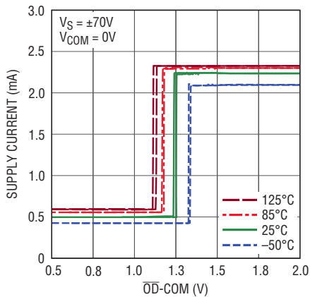
Supply Current vs \overline{\text{OD}} Pin Voltage
