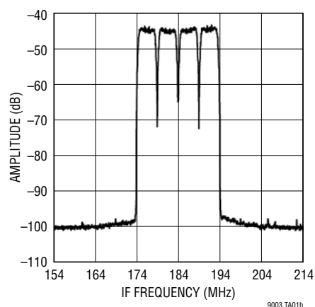
FFT of 4-Channel WCDMA Input at 2.14GHz
