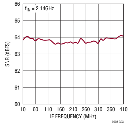
SNR vs Frequency, LTM9003-AA
