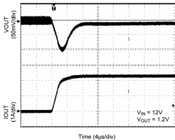
Transient Response
