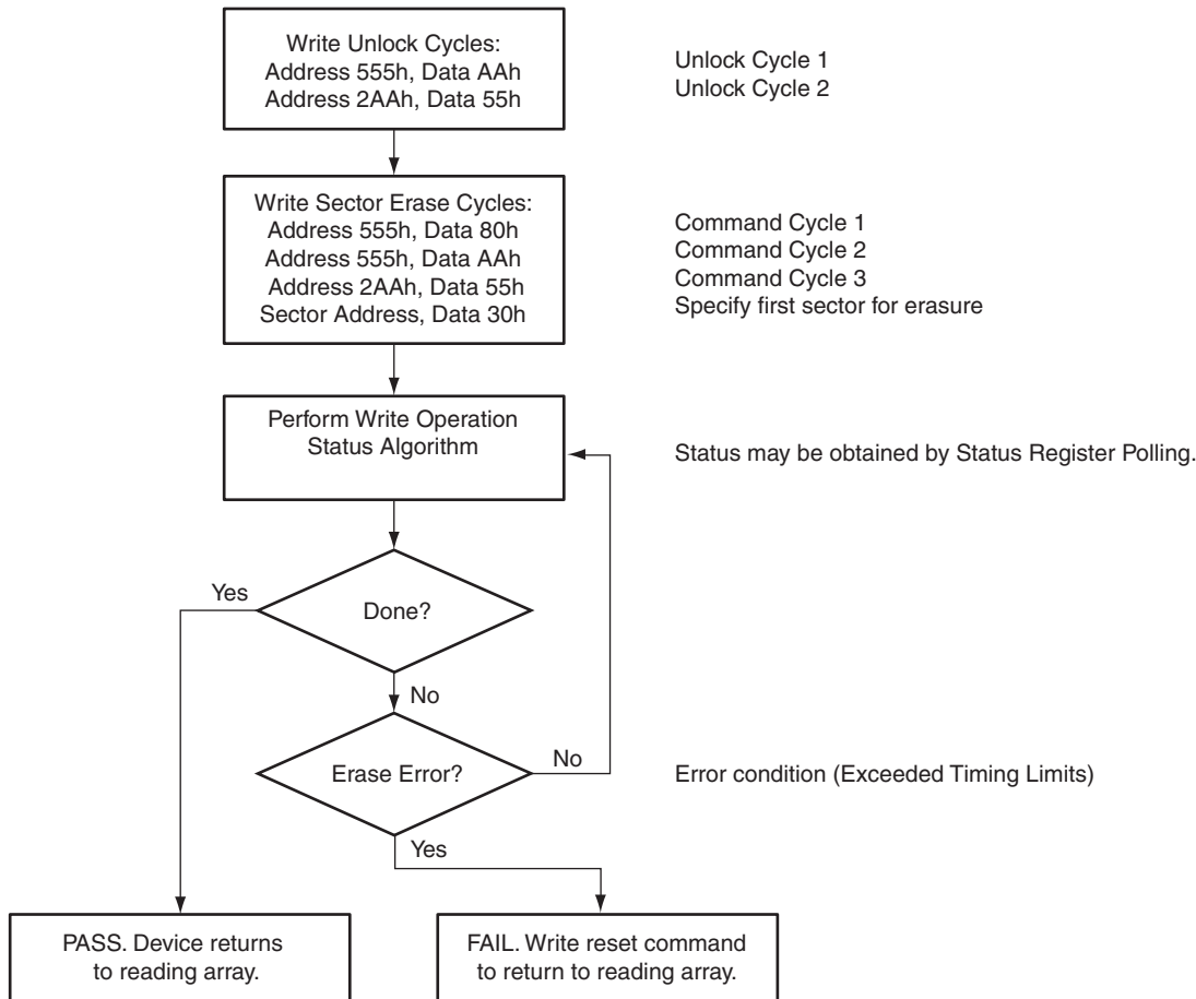
Figure 16. Sector Erase Operation
