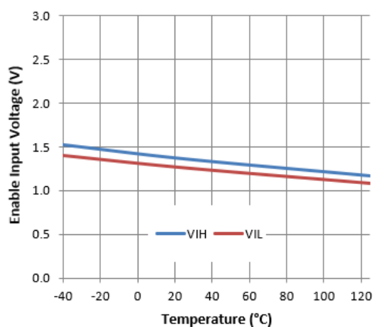
Fig 23. Enable Input Voltage vs. Temperature
