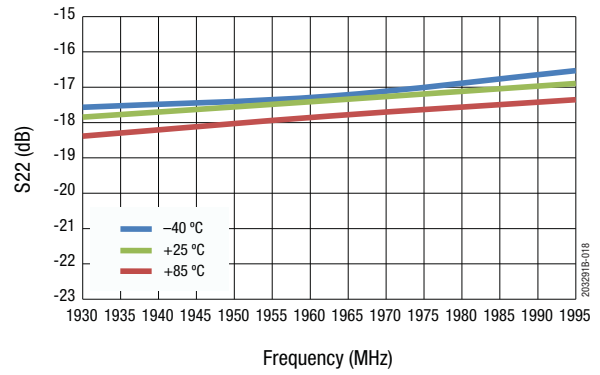
Figure 18. Output Return Loss vs Frequency at Different Temperature (Small Signal, P_{IN} = -20 dBm)
