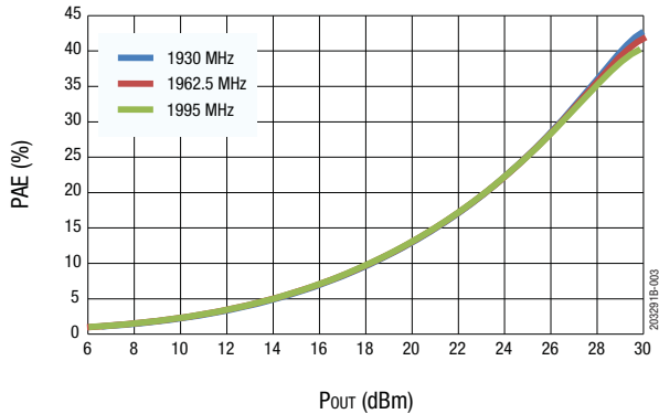
Figure 3. PAE vs Pout at Different Frequency
