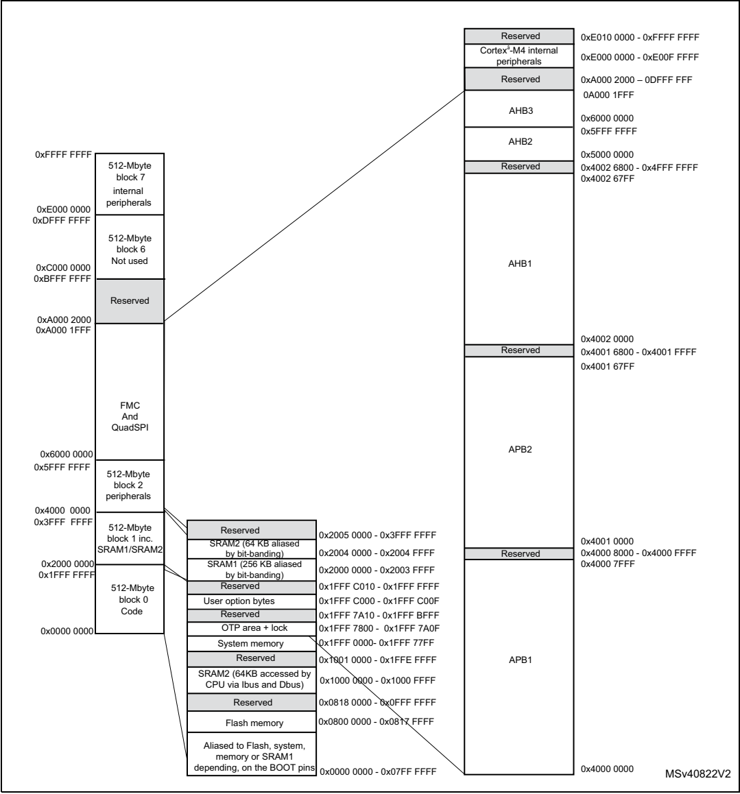
Figure 18. Memory map
