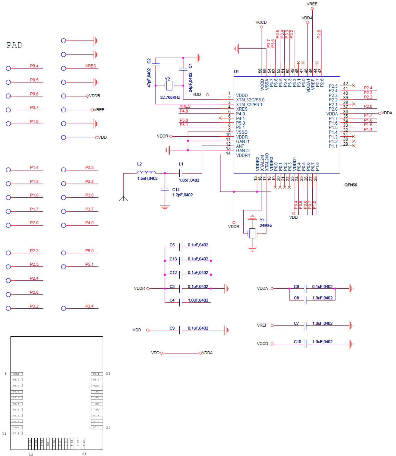
Figure 9. CYBLE-212019-00 Schematic Diagram
