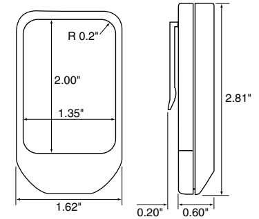
Figure 1: Package Dimensions
