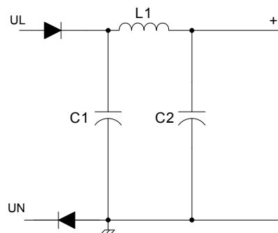
Figure 10: Half-Wave Rectifier
