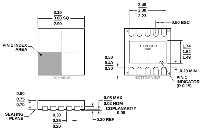
Figure 34. 10-Lead Lead Frame Chip Scale Package [LFCSP_WD] 3 mm × 3 mm Body, Very Very Thin, Dual Lead (CP-10-9)
