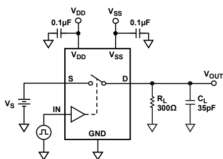
Figure 26. Switching Times
