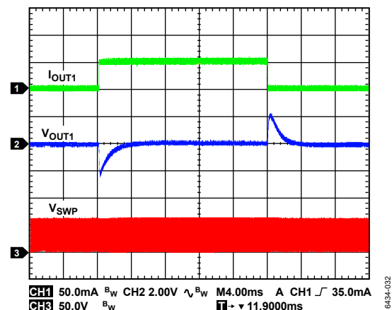
Figure 33. Flyback Regulator Load Transient Response, V_{INP} = 32\text{ V} , V_{OUT1} = 24\text{ V} , I_{OUT1} = 1\text{ mA} to 50\text{ mA} Step, T_A = 25^\circ\text{C}
