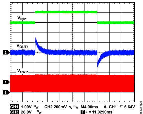
Figure 30. Flyback Regulator Line Transient Response, V_{INP} = 6\text{ V} to 7\text{ V} Step, V_{OUT1} = 24\text{ V} , I_{OUT1} = 20\text{ mA} , T_A = 25^\circ\text{C}
