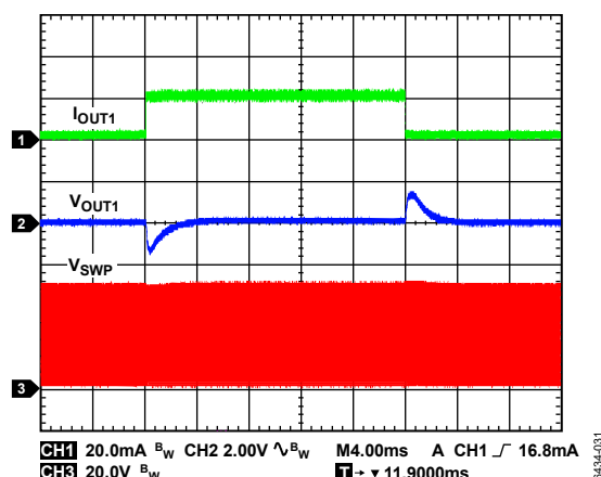
Figure 32. Flyback Regulator Load Transient Response, V_{INP} = 24\text{ V} , V_{OUT1} = 24\text{ V} , I_{OUT1} = 1\text{ mA} to 20\text{ mA} Step, T_A = 25^\circ\text{C}
