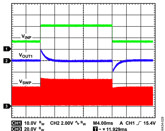
Figure 29. Flyback Regulator Line Transient Response, V_{INP} = 6\text{ V} to 20\text{ V} Step, V_{OUT1} = 24\text{ V} , I_{OUT1} = 20\text{ mA} , T_A = 25^\circ\text{C}
