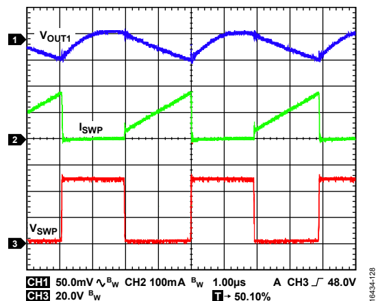
Figure 28. Flyback Regulator Continuous Conduction Mode Operation Showing I_{SWP} , Switch Node Voltage, and Output Ripple, T_A = 25^\circ\text{C} , V_{INP} = 24\text{ V} , V_{OUT1} = 24\text{ V} , I_{OUT1} = 50\text{ mA}
