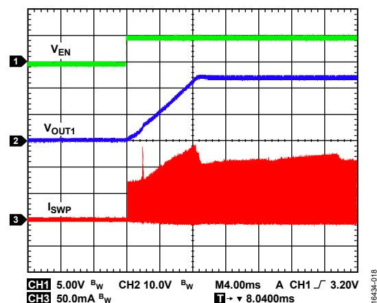
Figure 19. Inrush Current, T_A = +25^\circ\text{C} , V_{\text{INP}} = +24\text{ V} , V_{\text{OUT1}} = +24\text{ V} , I_{\text{OUT1}} = +20\text{ mA} , V_{\text{OUT2}} = +5.15\text{ V} , I_{\text{OUT2}} = +7\text{ mA} , V_{\text{OUT3}} = -15\text{ V} , I_{\text{OUT3}} = -0.3\text{ mA}
