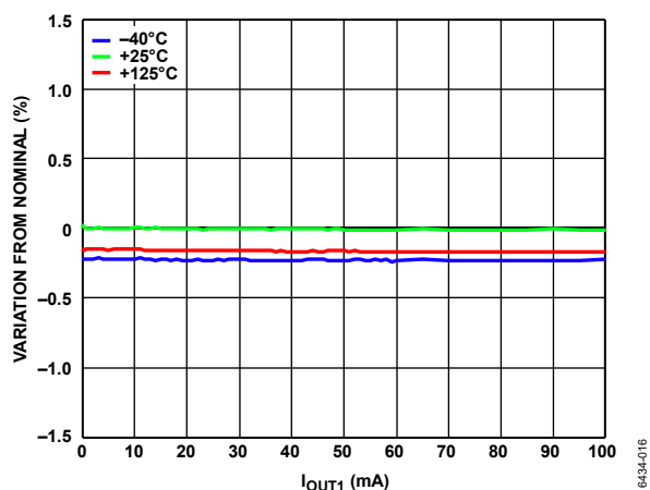
Figure 17. Flyback Regulator Load Regulation Across Temperature, V_{\text{INP}} = 24\text{ V} , V_{\text{OUT1}} = 24\text{ V} , Nominal = V_{\text{OUT1}} at 20 mA Load
