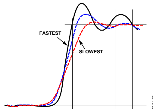
Figure 65. Switching Node at Various Slew Rate Settings
