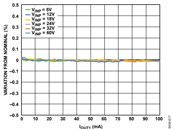
Figure 18. Flyback Regulator Load Regulation at Various Input Voltages, T_A = 25^\circ\text{C} , V_{\text{OUT1}} = 24\text{ V} , Nominal = V_{\text{OUT1}} at 20 mA Load
