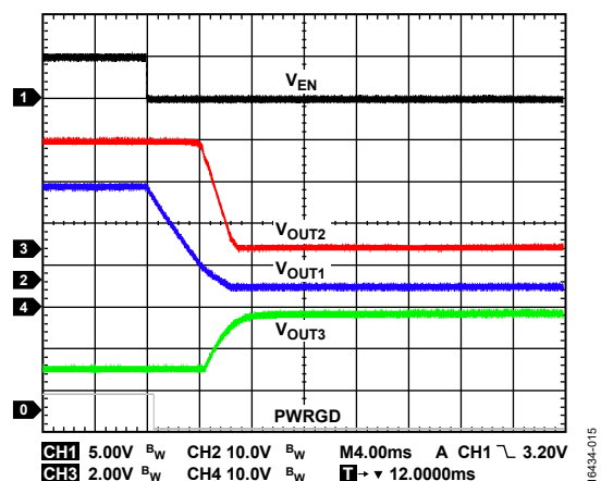
Figure 16. Shutdown Sequence, T_A = +25^\circ\text{C} , V_{\text{INP}} = +24\text{ V} , V_{\text{OUT1}} = +24\text{ V} , I_{\text{OUT1}} = +20\text{ mA} , V_{\text{OUT2}} = +5.15\text{ V} , I_{\text{OUT2}} = +7\text{ mA} , V_{\text{OUT3}} = -15\text{ V} , I_{\text{OUT3}} = -0.3\text{ mA}
