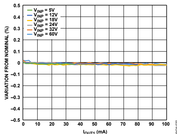
Figure 21. Flyback Regulator Load Regulation at Various Input Voltages, T_A = 25^\circ\text{C} , V_{\text{OUT1}} = 21\text{ V} , Nominal = V_{\text{OUT1}} at 20 mA Load
