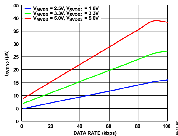
Figure 61. I_{SVDD2} Supply Current ( I_{SVDD2} ) vs. Data Rate on All GPIO Channels at Various Supply Voltages, \overline{MSS} Is High
