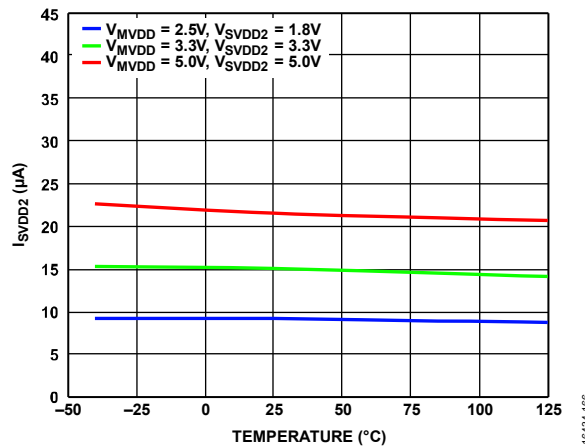
Figure 62. I_{SVDD2} vs. Temperature at Various Supply Voltages, \overline{MSS} Is Low, Data Rate = 40 kbps on All GPIO Channels
