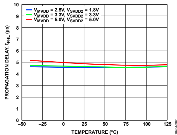
Figure 63. GPIO Channels Propagation Delay ( t_{PHL} ) vs. Temperature at Various Supply Voltages
