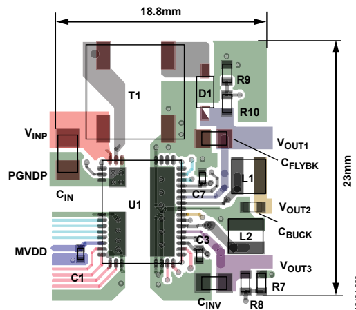
Figure 77. Suggested Top Layer Layout
