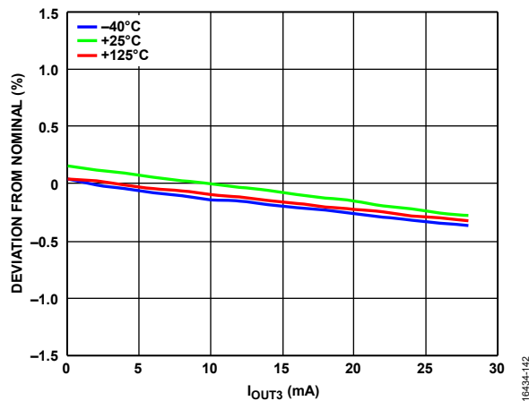
Figure 41. Inverting Regulator Load Regulation Across Temperature, V_{OUT1} = +24\text{ V} , V_{OUT3} = -15\text{ V} , Nominal = V_{OUT3} at -7\text{ mA} I_{OUT3}
