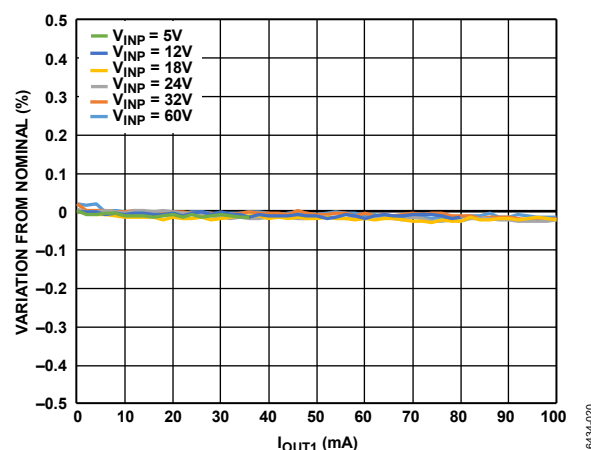
Figure 21. Flyback Regulator Load Regulation at Various Input Voltages, T_A = 25^\circ\text{C} , V_{OUT1} = 21\text{ V} , Nominal = V_{OUT1} at 20 mA Load
