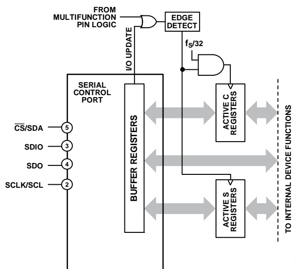
Figure 68. Buffered and Active Registers
