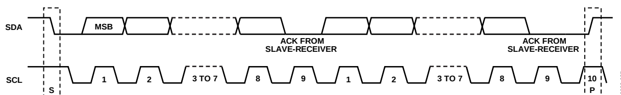
Figure 64. Acknowledge Bit
