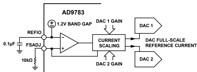
Figure 32. Reference Circuitry
