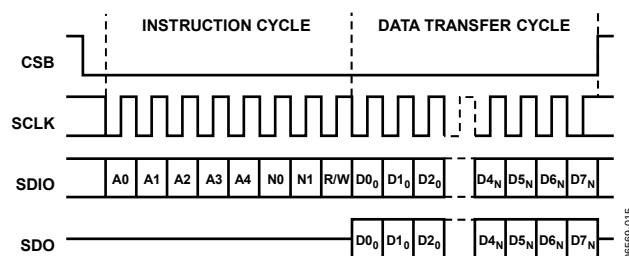
Figure 23. Serial Register Interface Timing—LSB First
