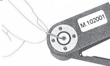
Figure 9: Conductor Insertion
