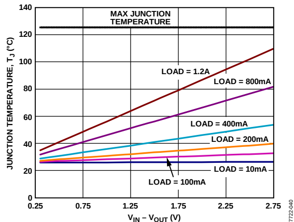
Figure 44. 1000 mm² of PCB Copper, T_B = 25^\circ\text{C} , LFCSP
