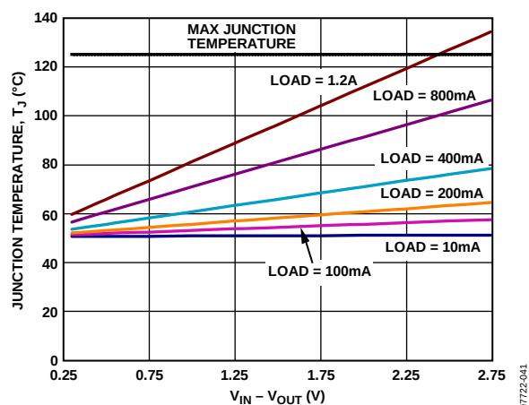
Figure 45. 1000 mm² of PCB Copper, T_B = 50^\circ\text{C} , LFCSP
