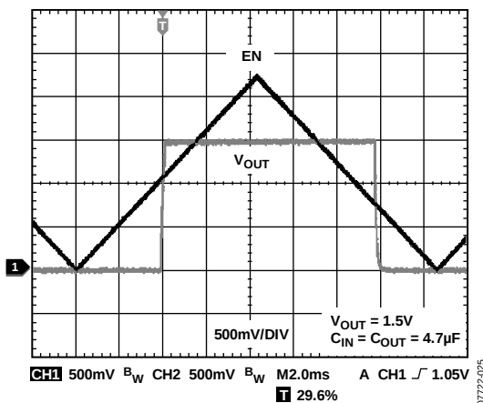
Figure 28. Typical EN Pin Operation
