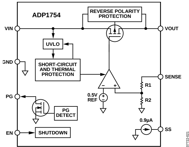
Figure 24. ADP1754 Internal Block Diagram
