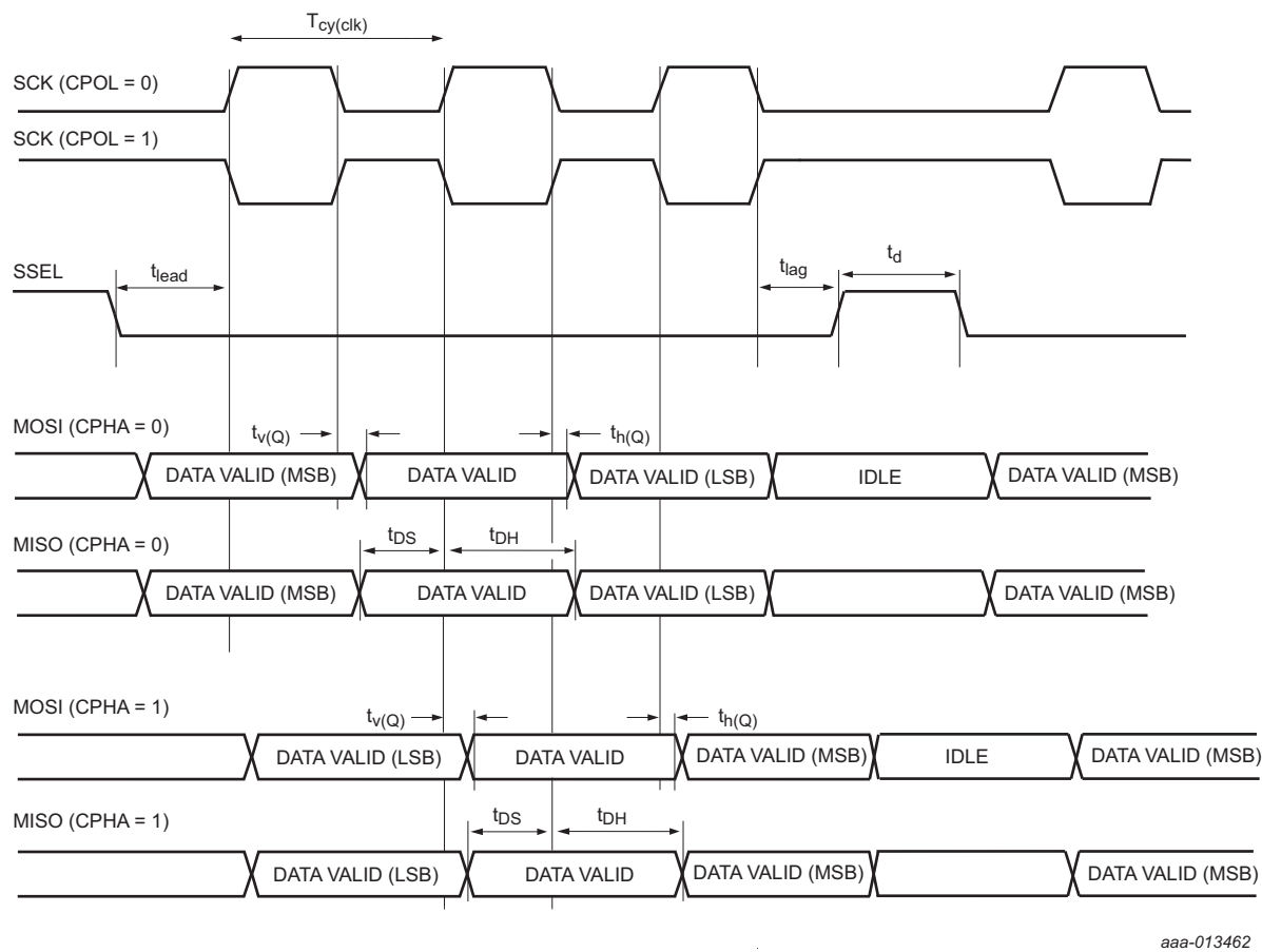
Fig 28. SSP_master mode timing (SPI mode)
