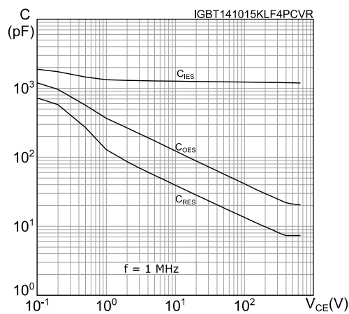
Figure 14: Capacitance variations
