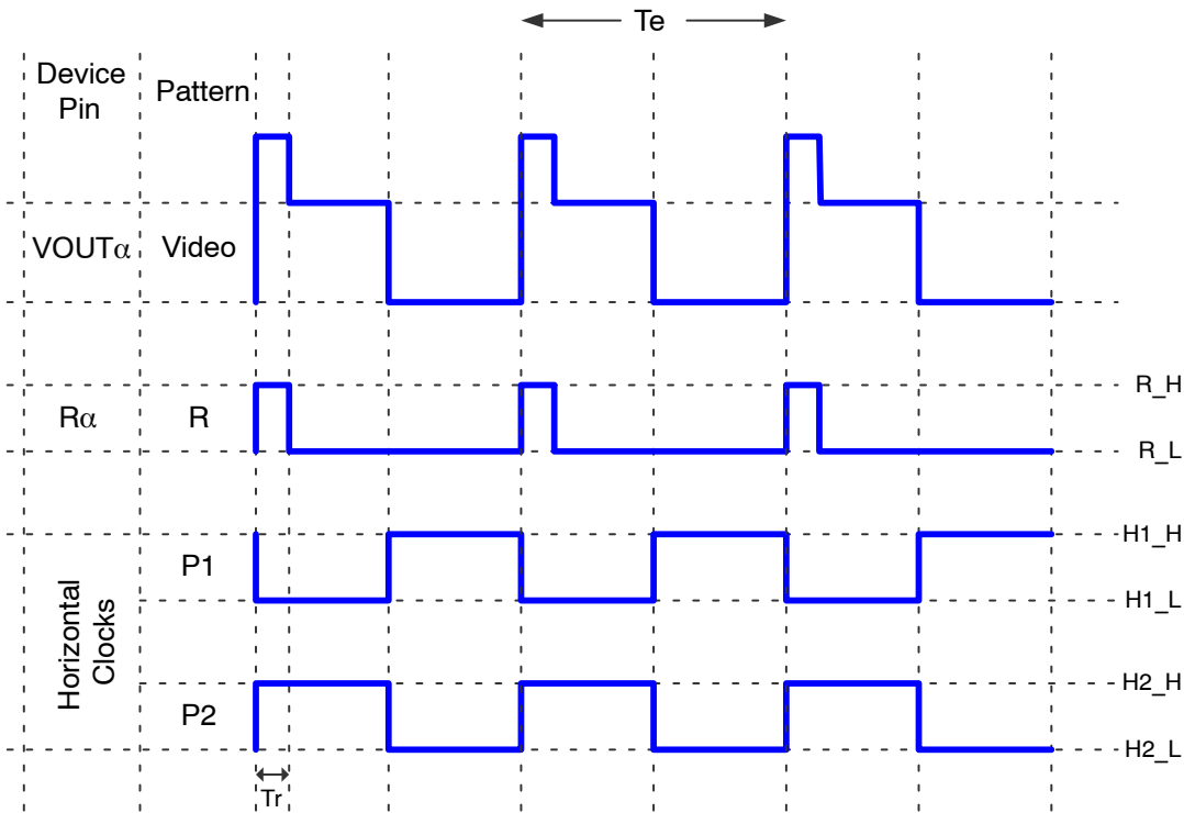
Figure 27. Pixel Timing Diagram – Full Resolution
