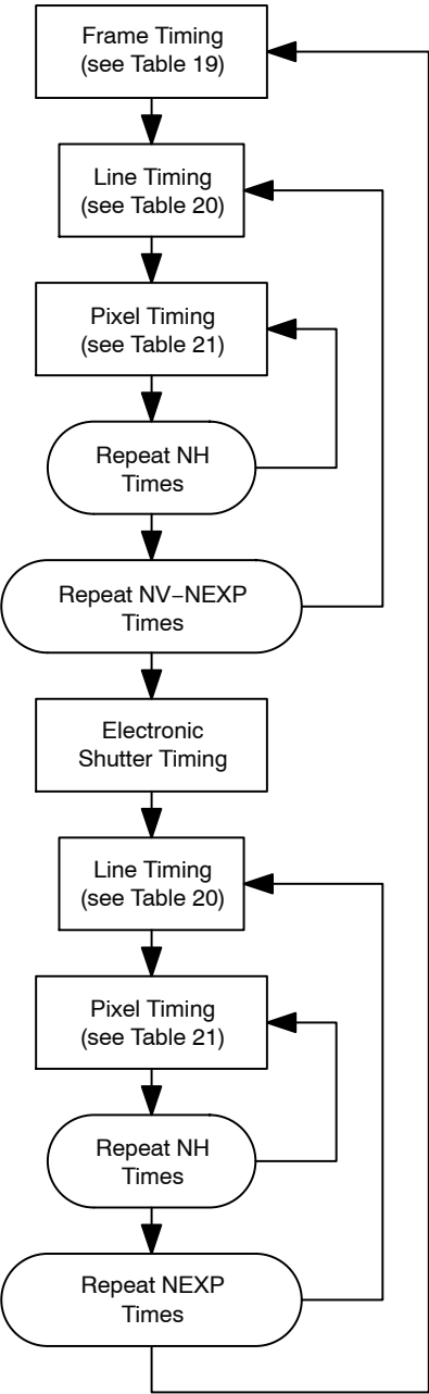
Figure 20. Timing Flow Chart using the Electronic Shutter for Exposure Control
