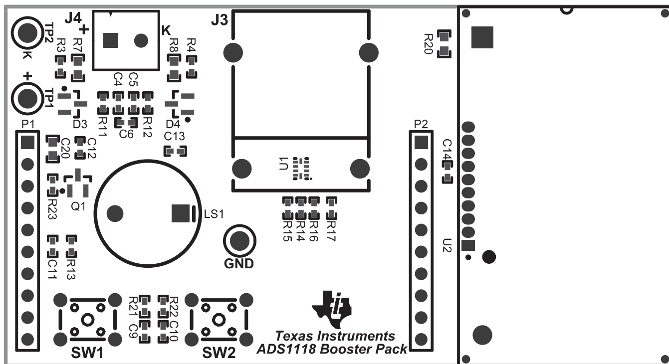
Figure 14. Top-Layer Silkscreen
