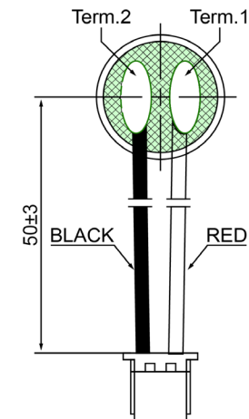
BOTTOM VIEW
