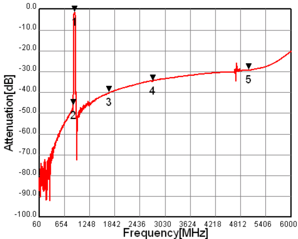
Fig.4 Wide-band Characteristics
