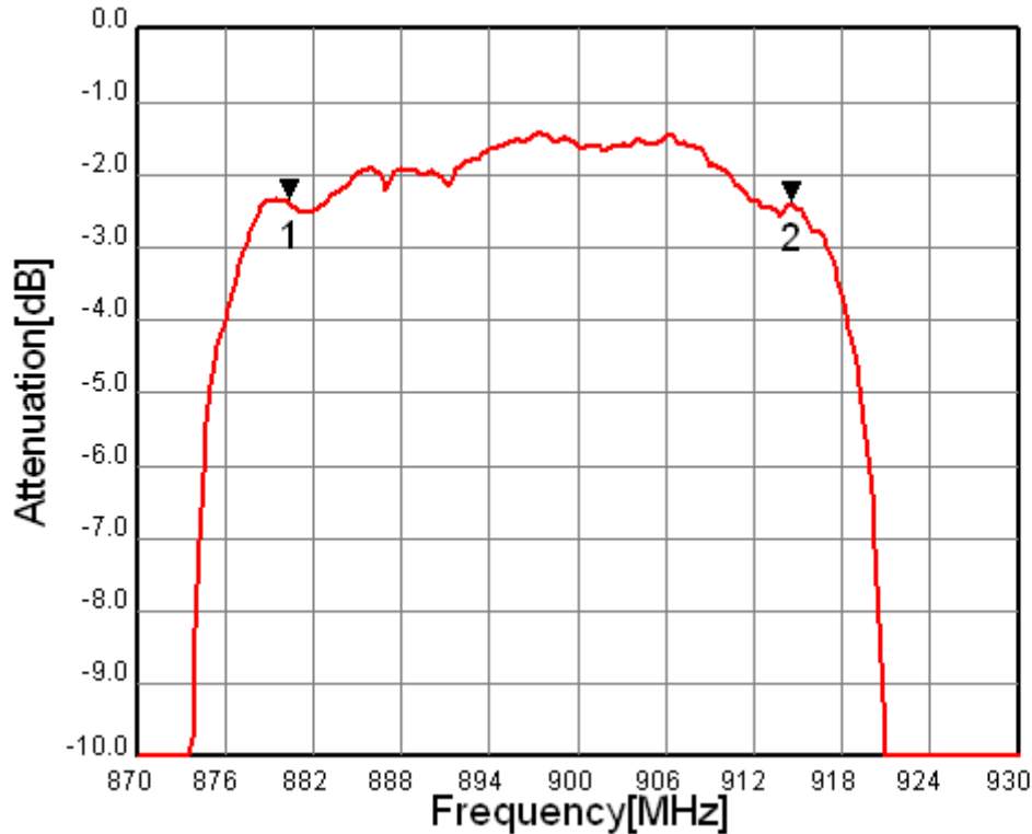
Fig.3 In-band Characteristics
