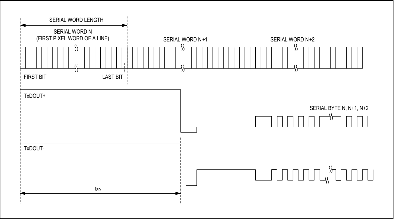
Figure 8. Deserializer Delay
