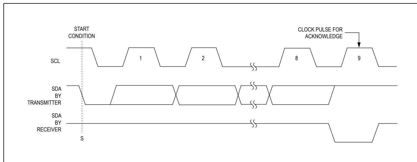
Figure 49. Acknowledge
