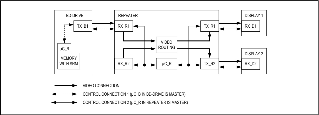
Figure 58. Example Network with One Repeater and Two μCs (Tx = GMSL Serializer's, Rx = Deserializer's)
