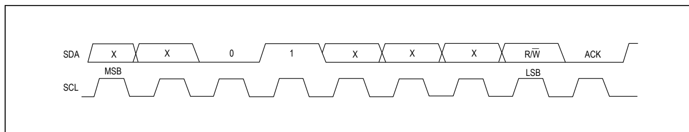
Figure 50. Slave Address
