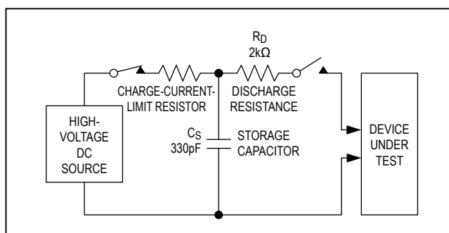
Figure 61. ISO 10605 Contact Discharge ESD Test Circuit
