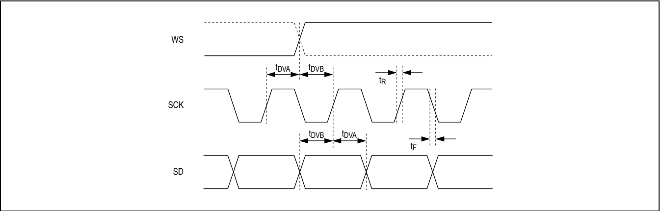
Figure 12. Output I2S Timing Parameters
