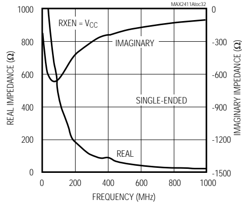
IF OR \bar{I}F OUTPUT IMPEDANCE vs. FREQUENCY
