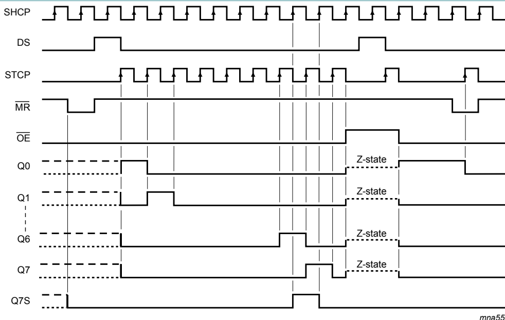
Figure 7. Timing diagram
