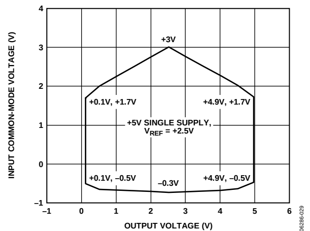
Figure 28. Input Common-Mode Voltage Range vs. Output Voltage, G = 100 , V_S = 5\text{ V} , V_{REF} = 2.5\text{ V}
