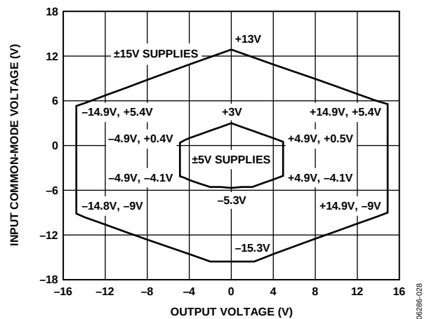
Figure 27. Input Common-Mode Voltage Range vs. Output Voltage, G = 100 , V_{REF} = 0\text{ V}
