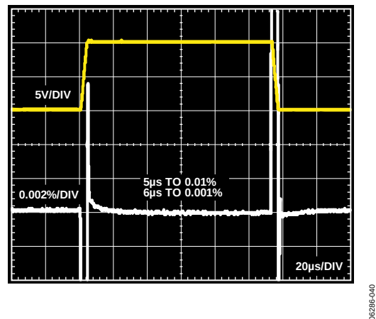
Figure 39. Large Signal Pulse Response and Settle Time, G = 1 , R_{LOAD} = 10\text{ k}\Omega , V_S = \pm 15\text{ V} , V_{REF} = 0\text{ V}
