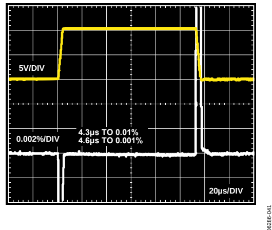
Figure 40. Large Signal Pulse Response and Settle Time, G = 10 , R_{LOAD} = 10\text{ k}\Omega , V_S = \pm 15\text{ V} , V_{REF} = 0\text{ V}
