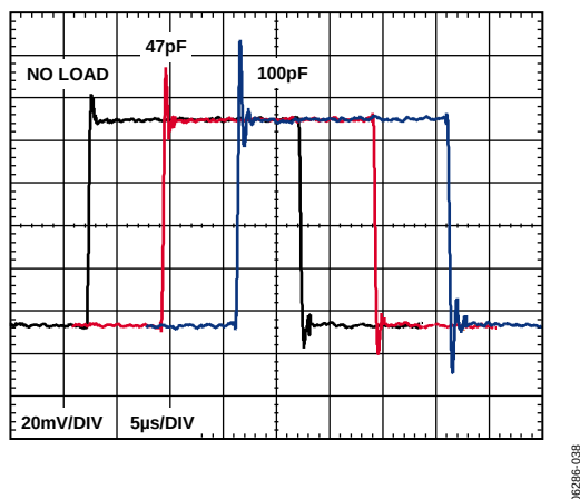
Figure 37. Small Signal Pulse Response for Various Capacitive Loads, V_S = 5\text{ V} , V_{REF} = 2.5\text{ V}
