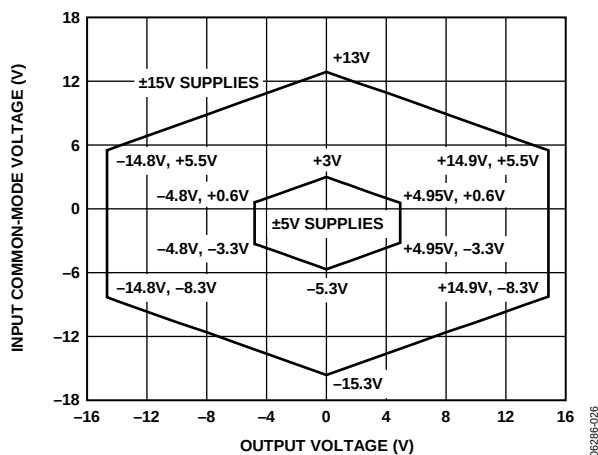
Figure 25. Input Common-Mode Voltage Range vs. Output Voltage, G = 1 , V_{REF} = 0\text{ V}
