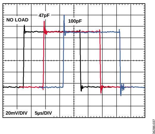
Figure 36. Small Signal Pulse Response for Various Capacitive Loads, V_S = \pm 15\text{ V} , V_{REF} = 0\text{ V}
