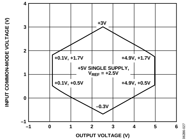
Figure 26. Input Common-Mode Voltage Range vs. Output Voltage, G = 1 , V_S = 5\text{ V} , V_{REF} = 2.5\text{ V}
