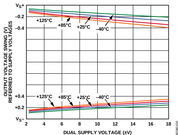
Figure 31. Output Voltage Swing vs. Dual Supply Voltage, R_{LOAD} = 10 kΩ, G = 10 , V_{REF} = 0 V
