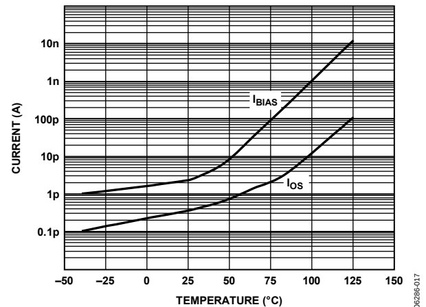
Figure 16. Input Bias Current and Offset Current vs. Temperature, V_S = 5\text{ V} , V_{REF} = 2.5\text{ V}
