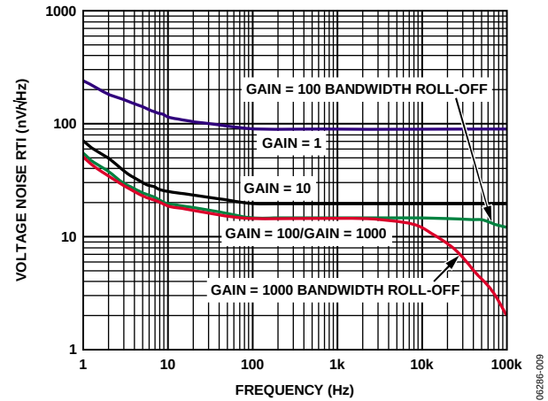
Figure 8. Voltage Spectral Density vs. Frequency
