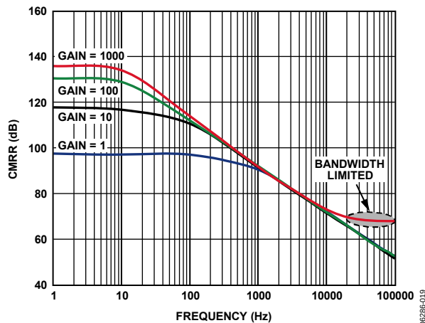
Figure 18. CMRR vs. Frequency, 1 k \Omega Source Imbalance
