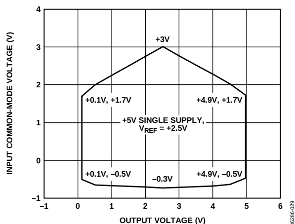
Figure 28. Input Common-Mode Voltage Range vs. Output Voltage, G = 100 , V_S = 5V , V_{REF} = 2.5V
