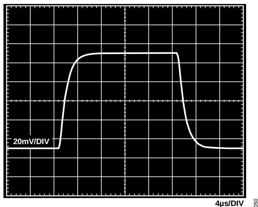
Figure 49. Small Signal Pulse Response, G = 100 , R_{LOAD} = 2\text{ k}\Omega , C_{LOAD} = 100\text{ pF} , V_S = 5\text{ V} , V_{REF} = 2.5\text{ V}
