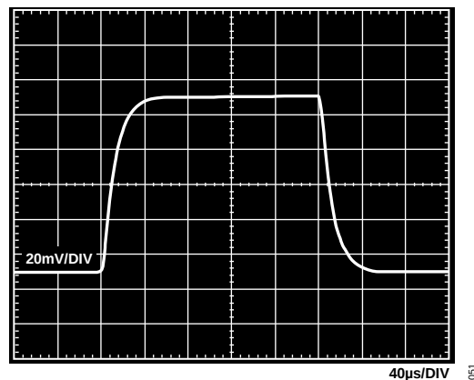
Figure 50. Small Signal Pulse Response, G = 1000 , R_{LOAD} = 2\text{ k}\Omega , C_{LOAD} = 100\text{ pF} , V_S = 5\text{ V} , V_{REF} = 2.5\text{ V}
