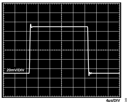
Figure 48. Small Signal Pulse Response, G = 10 , R_{LOAD} = 2\text{ k}\Omega , C_{LOAD} = 100\text{ pF} , V_S = 5\text{ V} , V_{REF} = 2.5\text{ V}
