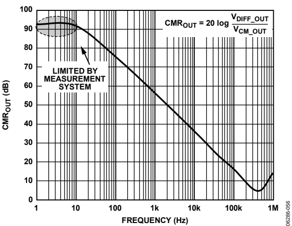
Figure 55. Differential Output Configuration: Common-Mode Output (CM OUT ) vs. Frequency
