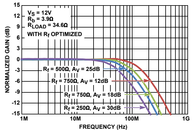
FIGURE 22. SMALL SIGNAL FREQUENCY RESPONSE vs GAINS
