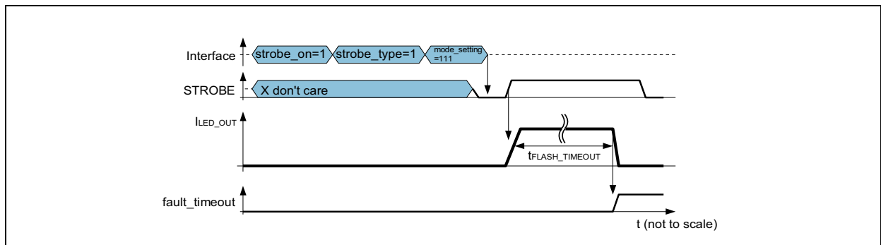
Figure AS3630 – 31: AS3630 Flash Duration and Start Defined by STROBE, Limited by flash_timeout; Timer Expired
