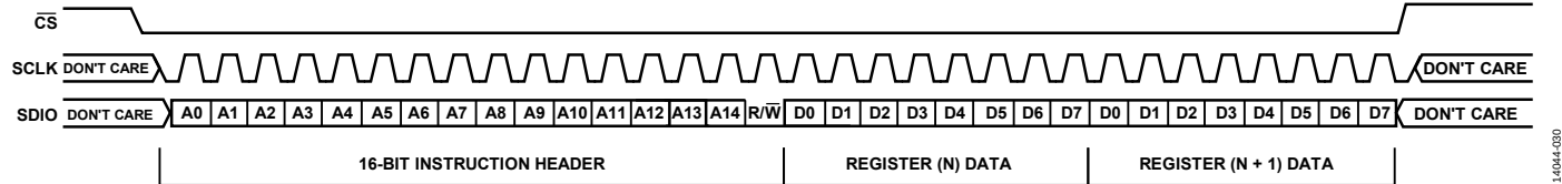
Figure 29. Serial Control Port Write—LSB First, Address Increment, Two Bytes of Data
