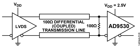
Figure 21. REFx Input Termination Recommendation for LVDS Drivers
