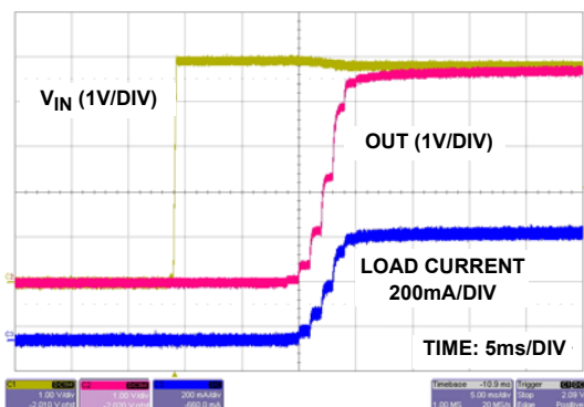
FIGURE 2. CAPTURED WAVEFORMS FOR POWER-UP. THE OUTPUT IS LOADED WITH A 10\Omega RESISTOR
