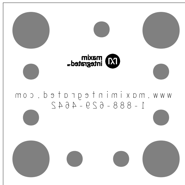
MAX40002–MAX40005 EV Kit—Bottom Silkscreen
