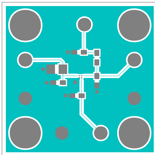
MAX40002–MAX40005 EV Kit—Top
