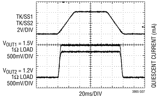
Tracking Up and Down with External Ramp (Forced Continuous Mode)
